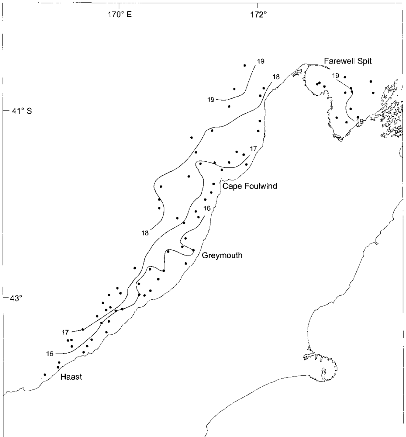
Figure 3: Positions of CTD sea surface temperature recordings and isotherms estimated from the temperature recordings.
